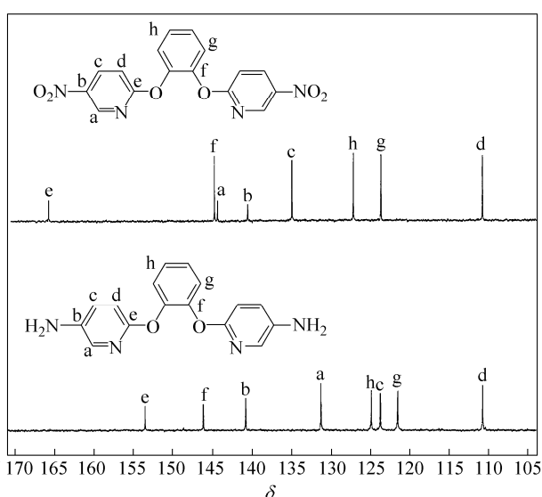
Fig. 3 ^{13}\text{C} -NMR spectra of o -PNP (top) and o -PAP (bottom)
