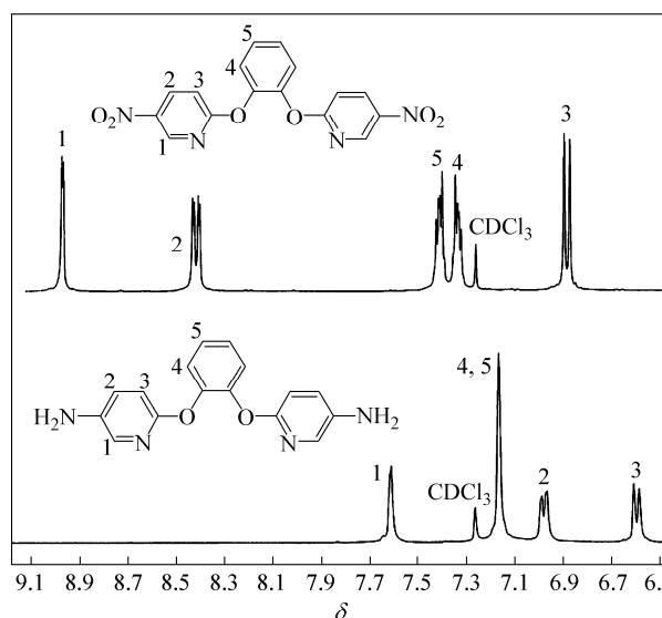
Fig. 2 ^1\text{H} -NMR spectra of o -PNP (top) and o -PAP (bottom)
